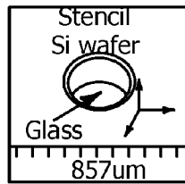
Glass wafer inflation through the hole.
