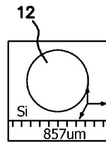
Final step. Spherical glass shell on stem.
