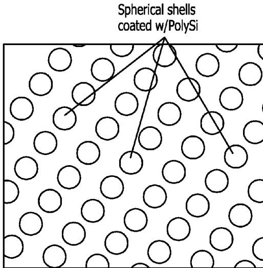
Array of glass-blown spherical shells on a wafer coated with polycrystalline silicon layer, Individual shell can be used a sensitive element of MSRSG.
