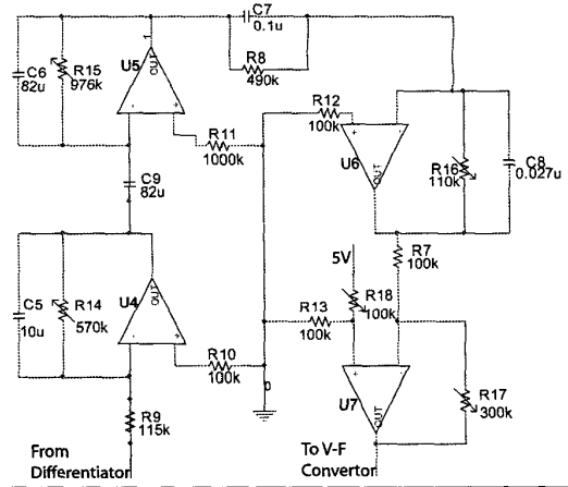
Fig. 2. Transfer function mimicking dynamics of the semicircular canals of the squirrel monkey model (reported in [7])
